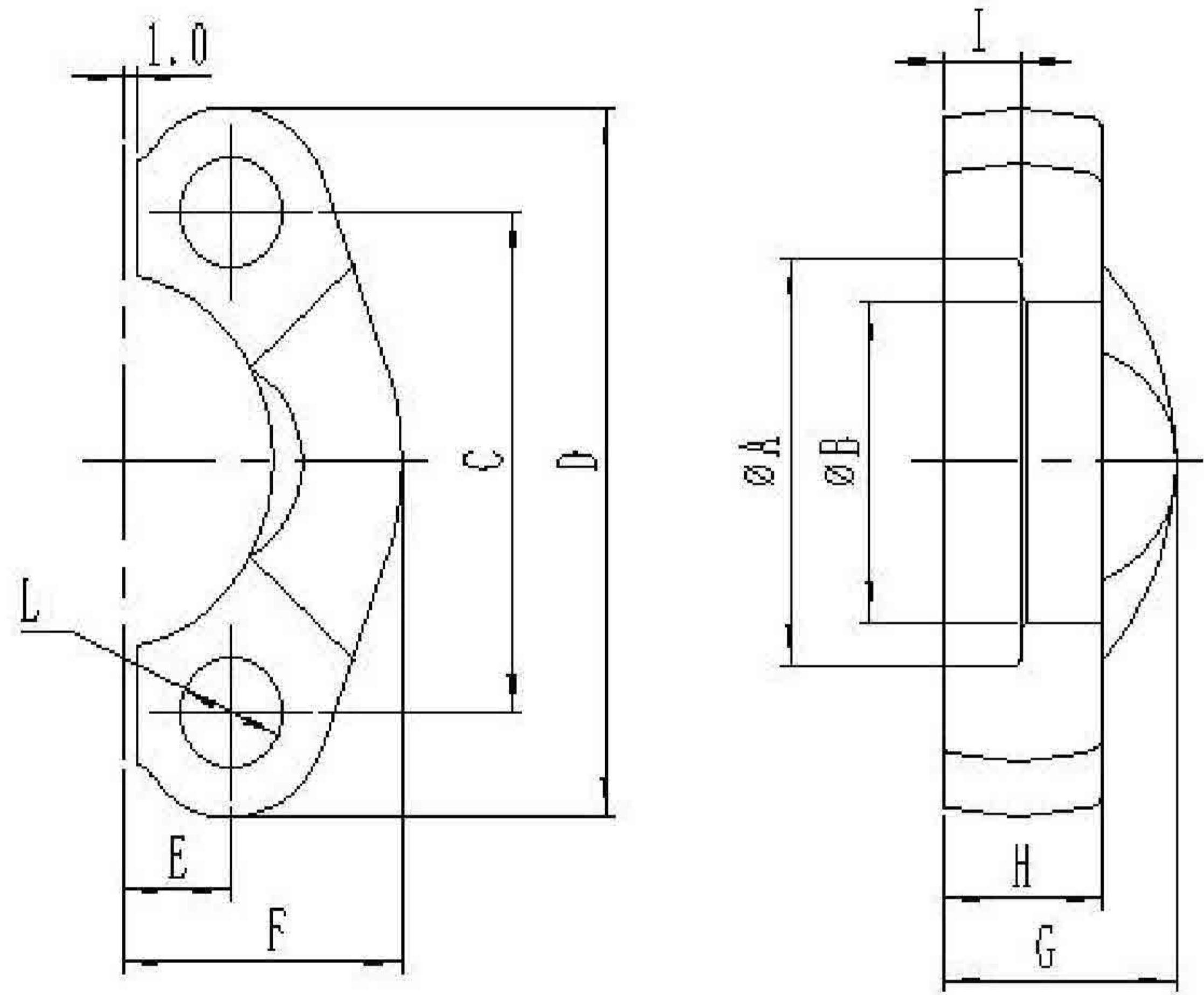
SAE split flang halves
