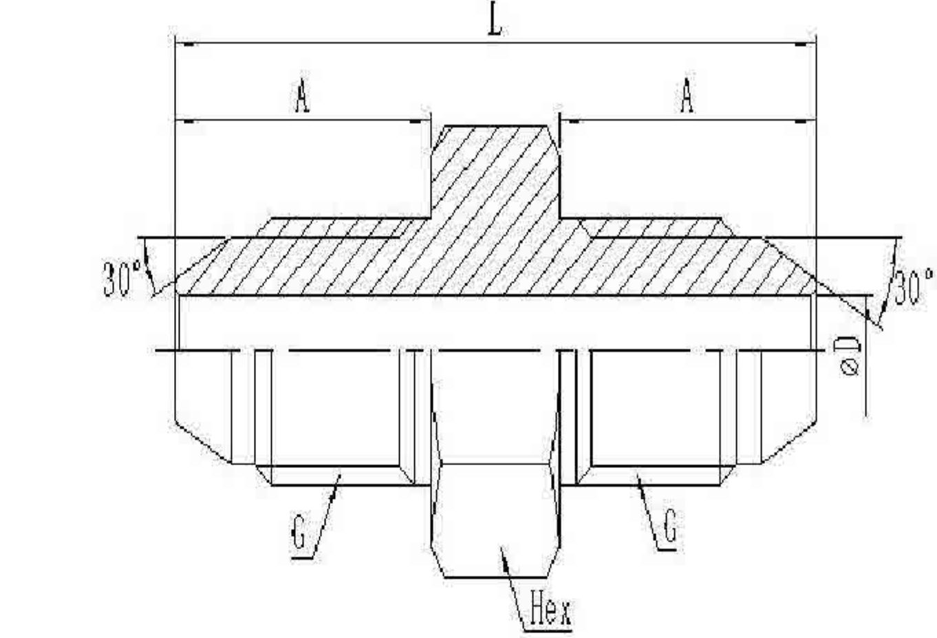
HEX NIPPLE 1014
