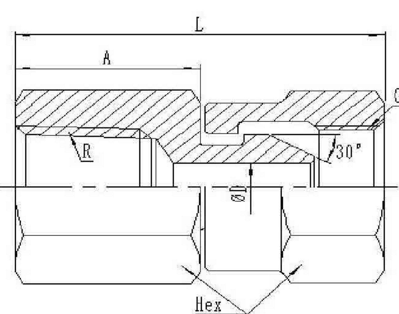
HEX NIPPLE 1008
