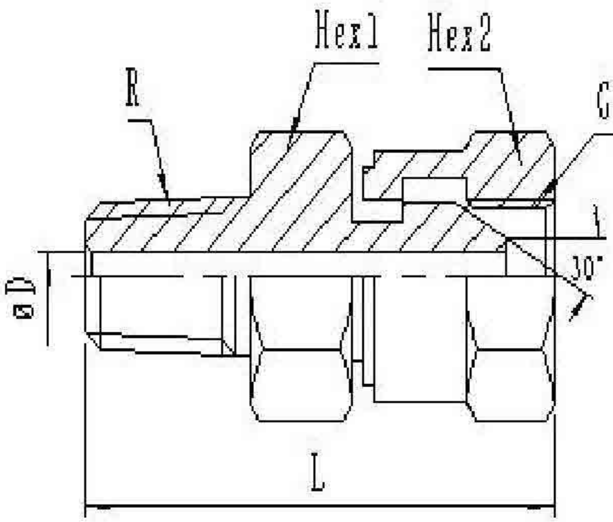
HEX NIPPLE 1006
